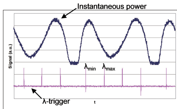
Figure 2. Instantaneous power (black) measured during swept operation, with starting/ending wavelength triggers (red).
